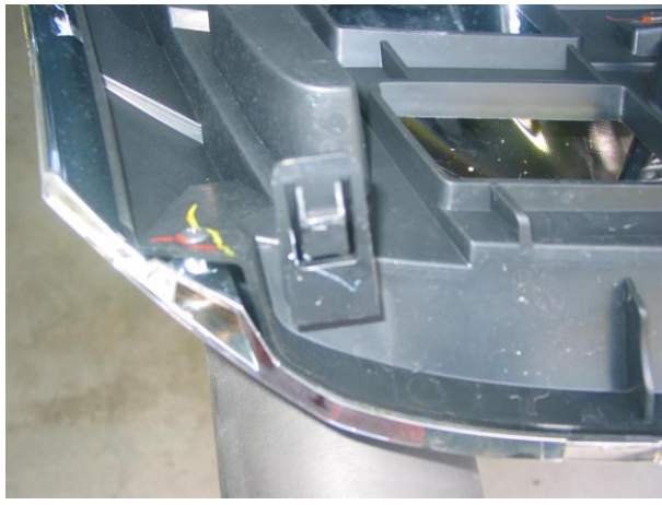
Figure 1: Lower outer clip on grille. Grille removed for photo.
